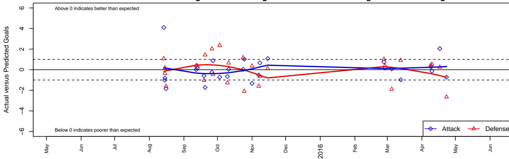
BSC Portland Gold-Tiempo B01 Dots are actual minus expected GF (blue circles) and GA (red triangles). Blue line is smoothed change in attack strength. Red is smoothed change in defense strength.
